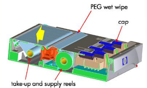
Print Head Cleaning Cartridge
